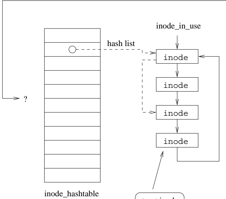
struct inode
